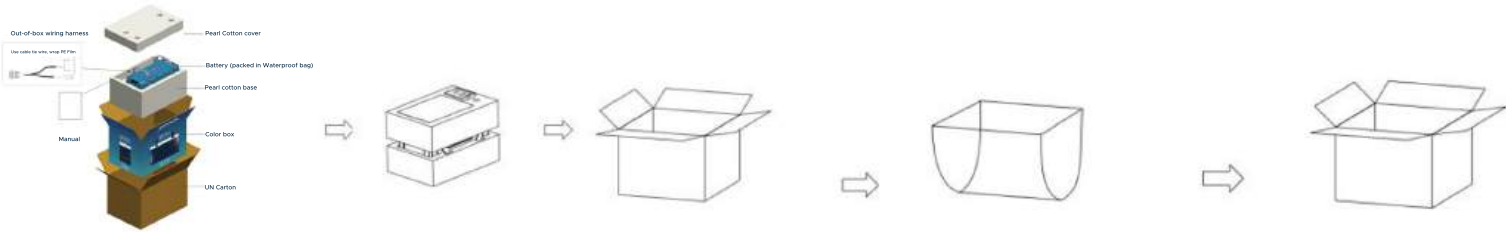
Figure 3. Schematic Diagram of Packaging
