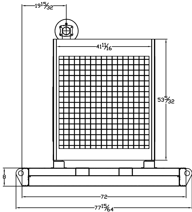
RADIATOR VIEW
